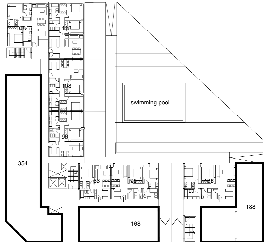
Piano Terra
